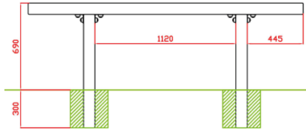
Vista Frontal
